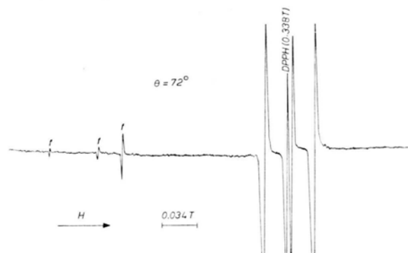
Fig. 1. ESR spectrum of \text{Cr}^{3+} in \text{AlCl}_3 \cdot 6\text{H}_2\text{O} single crystals at 308 K. Fine structure forbidden lines are marked f.
